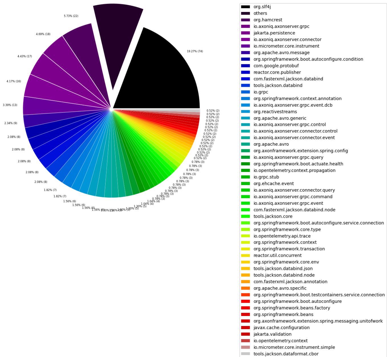
Top external package usage spread [%] by 8.77% (36)
