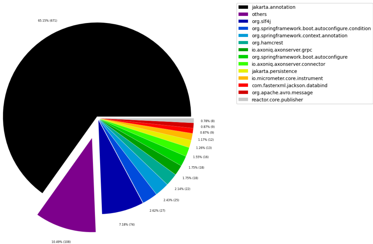
Top external package usage [%] by type (more than 0.7% overall)
