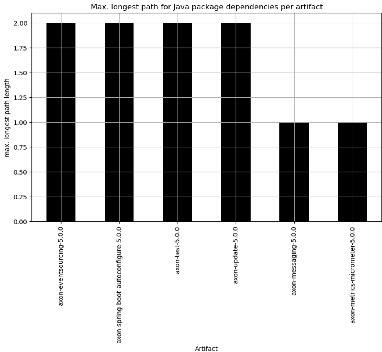
Longest path for each artifact - Bar chart (absolute)
