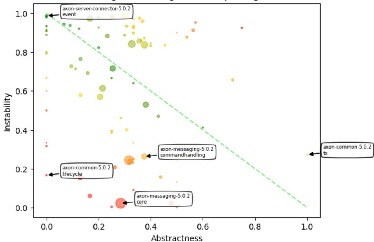
Abstractness vs. Instability ("Main Sequence") Packages including their sub-packages
