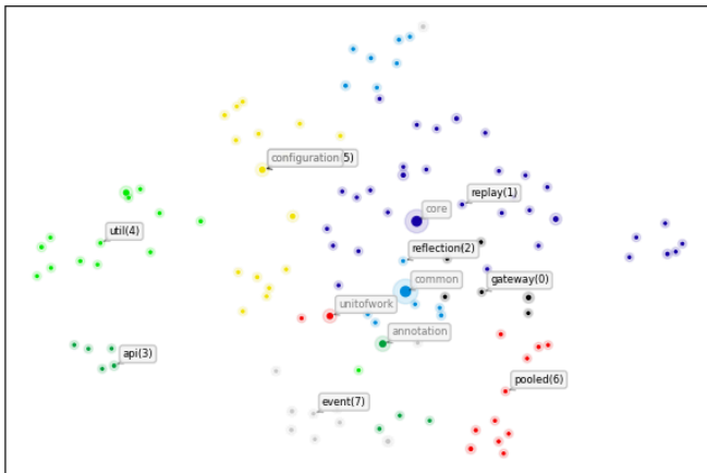
Java Packages dependency graph node embeddings Silhouette Score (aim higher)=0.2057, Davies-Bouldin Score (aim lower)=1.9299 node2vec -> UMAP
