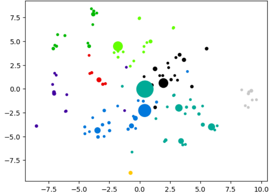
Java Package positioned by their dependency relationships (node2vec node embeddings + t-SNE)
