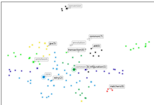
Java Packages dependency graph node embeddings Silhouette Score (aim higher)=0.2297, Davies-Bouldin Score (aim lower)=1.7395 node2vec -> UMAP
