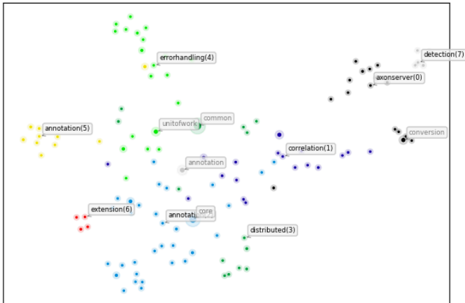
Java Packages dependency graph node embeddings Silhouette Score (aim higher)=0.2297, Davies-Bouldin Score (aim lower)=1.7395 node2vec -> UMAP
