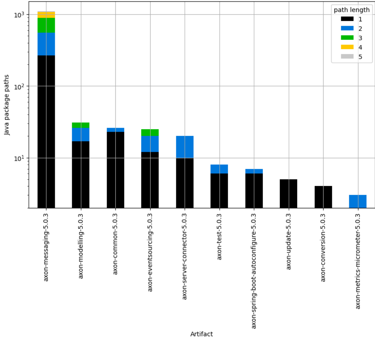
All pairs shortest path for Java package dependencies stacked per artifact (absolute, logarithmic)
