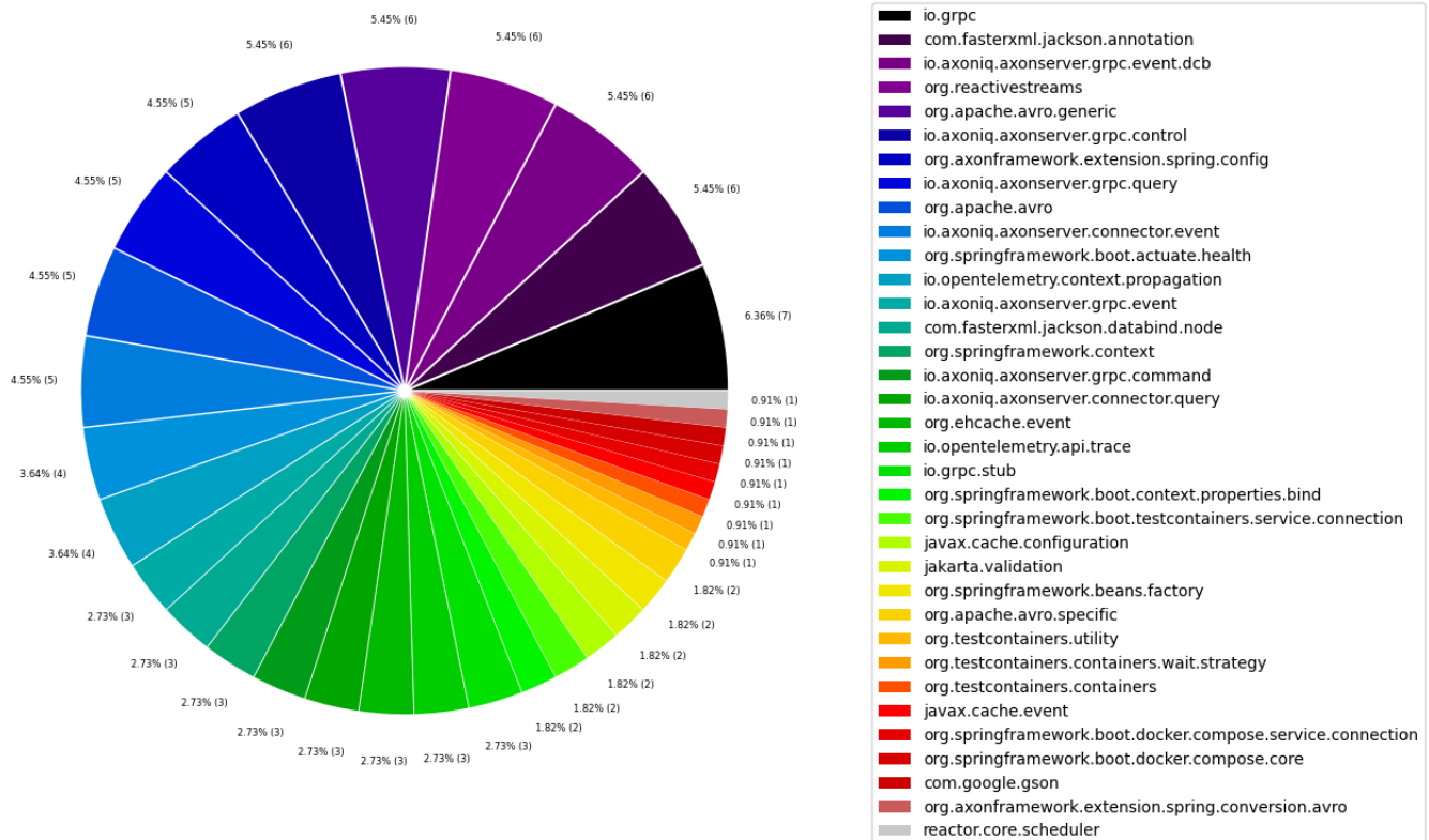
Top external package usage [%] by type (less than 0.7% overall "others" drill-down)
