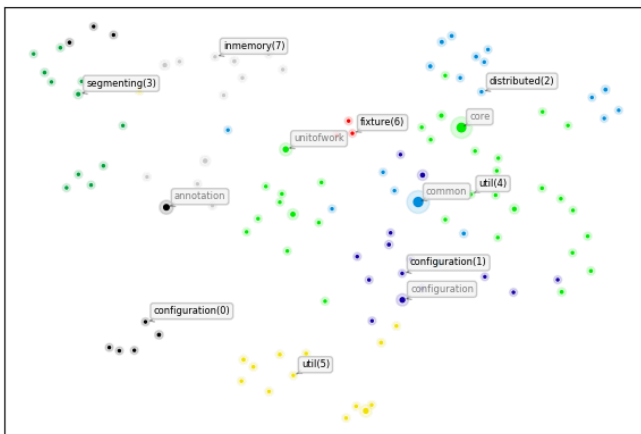
Java Packages dependency graph node embeddings Silhouette Score (aim higher)=0.2138, Davies-Bouldin Score (aim lower)=1.9084 node2vec -> UMAP
