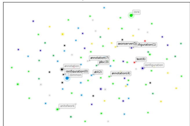
Java Packages dependency graph node embeddings Silhouette Score (aim higher)=-0.3997, Davies-Bouldin Score (aim lower)=0.0000 GraphSAGE -> UMAP
