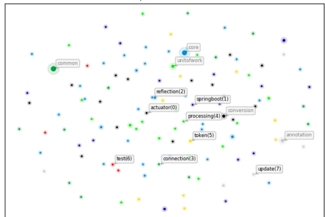
Java Packages dependency graph node embeddings Silhouette Score (aim higher)=-0.2575, Davies-Bouldin Score (aim lower)=0.0000 GraphSAGE -> UMAP
