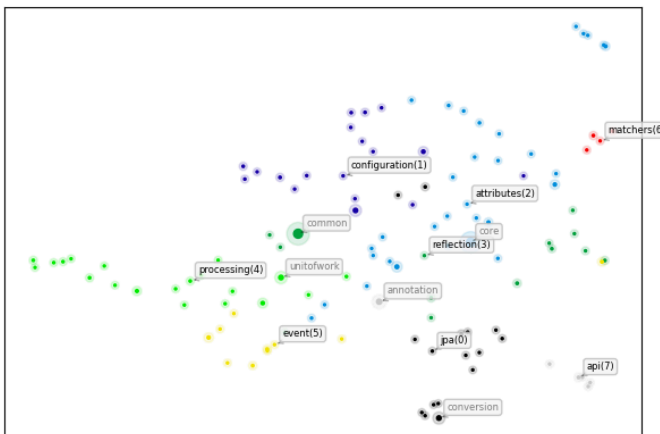
Java Packages dependency graph node embeddings Silhouette Score (aim higher)=0.2259, Davies-Bouldin Score (aim lower)=1.8011 node2vec -> UMAP
