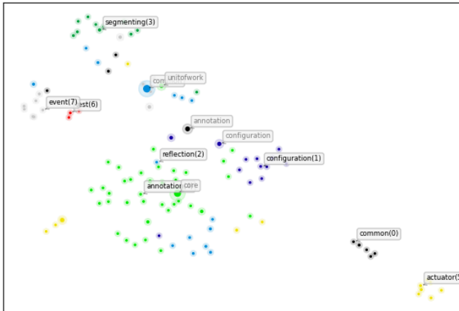
Java Packages dependency graph node embeddings Silhouette Score (aim higher)=0.2312, Davies-Bouldin Score (aim lower)=1.7847 node2vec -> UMAP
