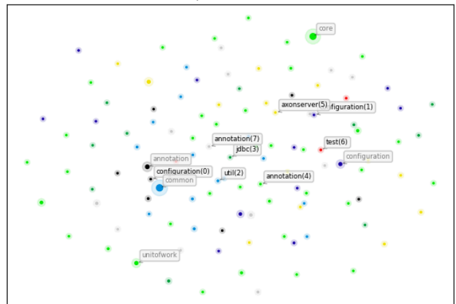
Java Packages dependency graph node embeddings Silhouette Score (aim higher)=-0.3917, Davies-Bouldin Score (aim lower)=0.0000 GraphSAGE -> UMAP
