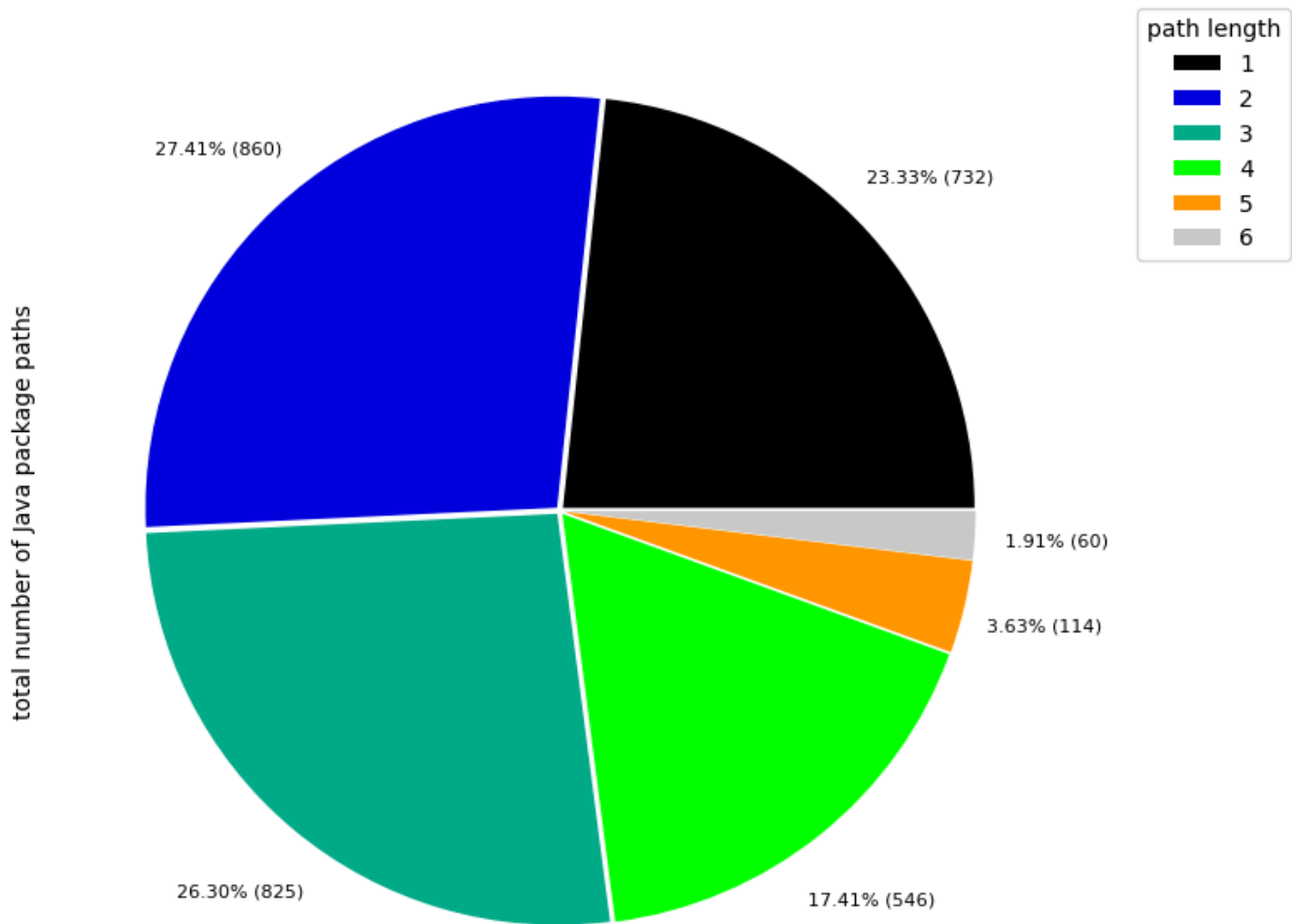
All pairs shortest path for Java package dependencies in total (pie)
