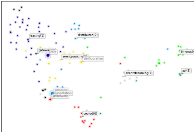
Java Packages dependency graph node embeddings Silhouette Score (aim higher)=0.2182, Davies-Bouldin Score (aim lower)=1.9127 node2vec -> UMAP
