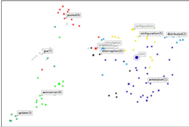
Java Packages dependency graph node embeddings Silhouette Score (aim higher)=0.1920, Davies-Bouldin Score (aim lower)=1.9991 node2vec -> UMAP
