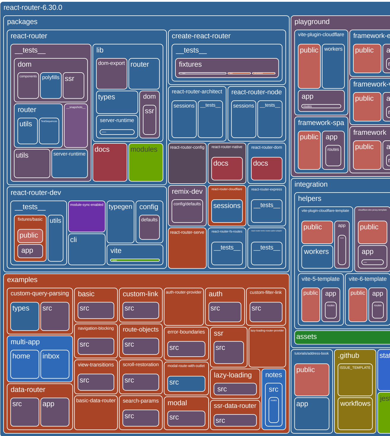
Most frequent file extension per directory
