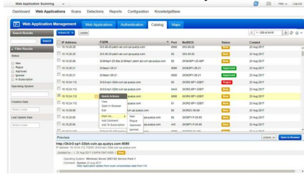
Scan Qualys
