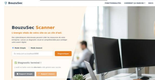
Interface BouzuSec
