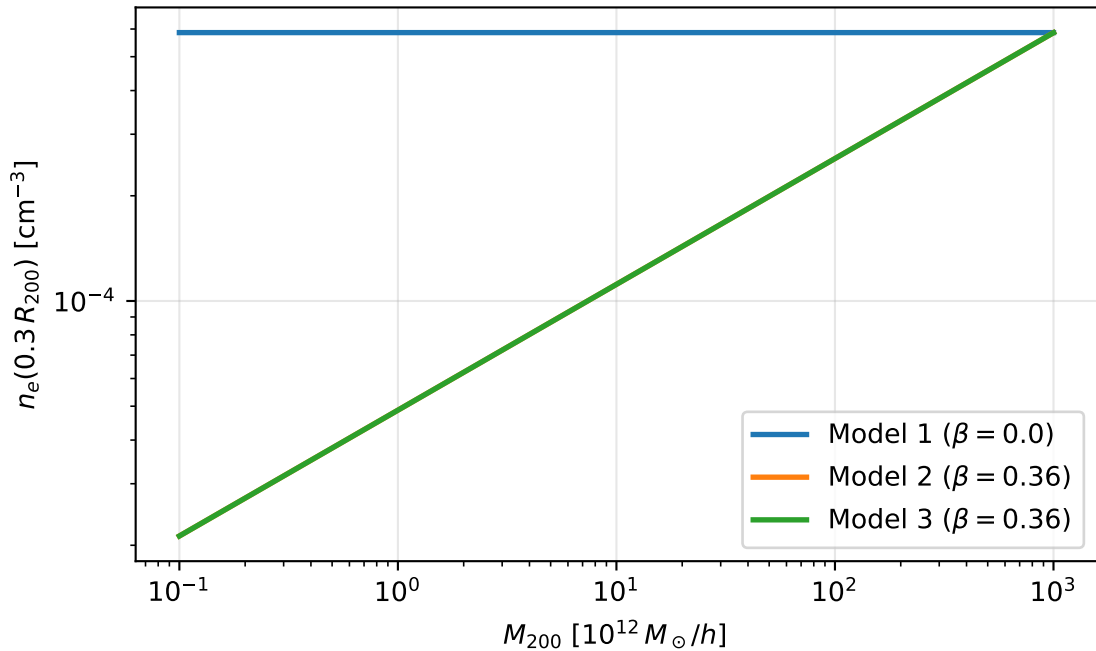
DPM mass scaling n_e \propto M_{200}^\beta at z = 0
