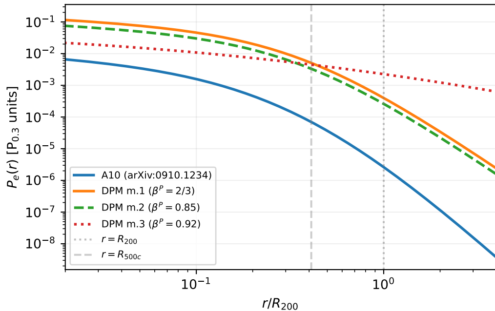
Electron pressure ( M_{200} = 10^{14} M_{\odot}/h , z = 0.1 )
