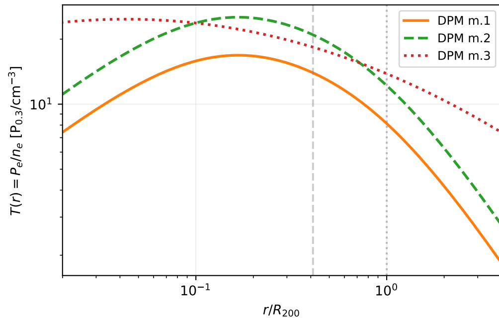
Temperature ( M_{200} = 10^{14} M_{\odot}/h , z = 0.1 )
