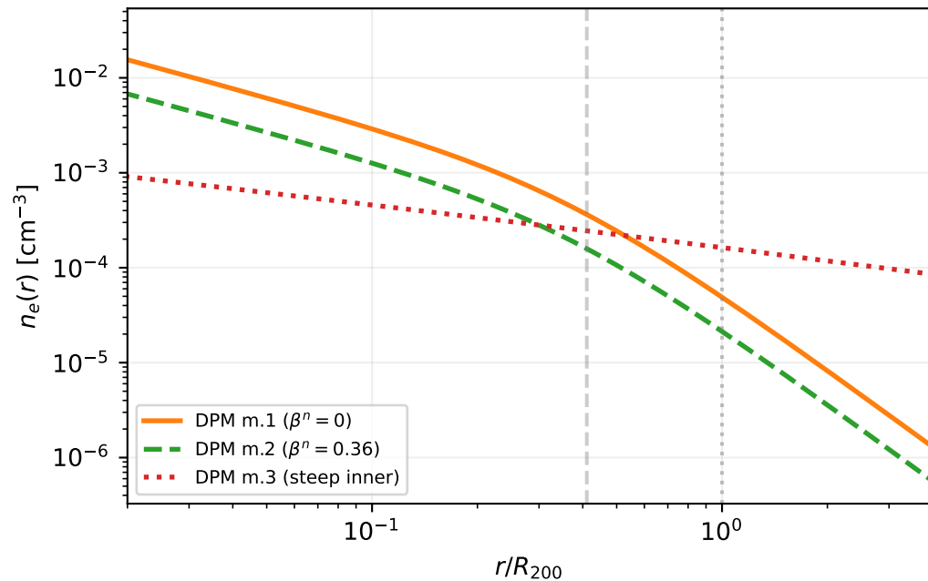
Electron density ( M_{200} = 10^{14} M_{\odot}/h , z = 0.1 )
