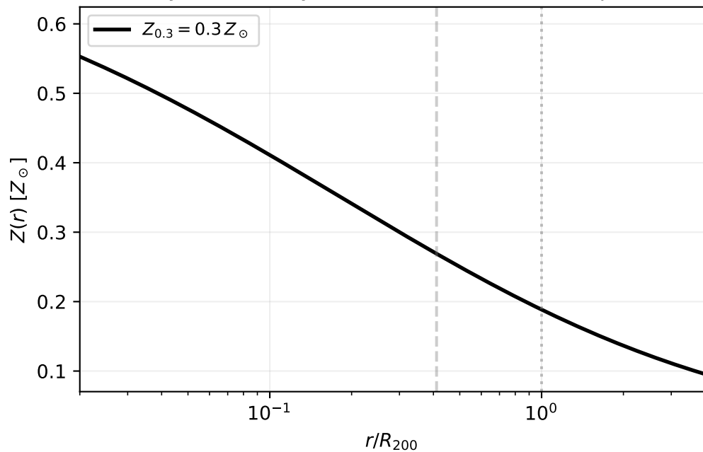
Metallicity (MetallicityProfileDPM, no mass/z dependence)
