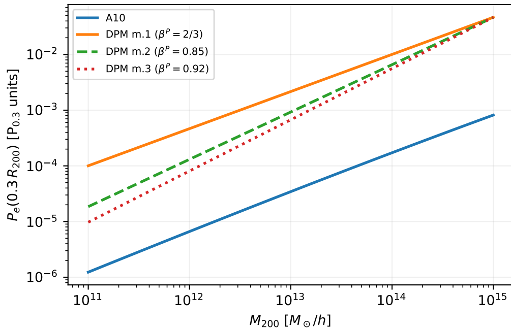
Pressure amplitude at r = 0.3 R_{200} , z = 0.1
