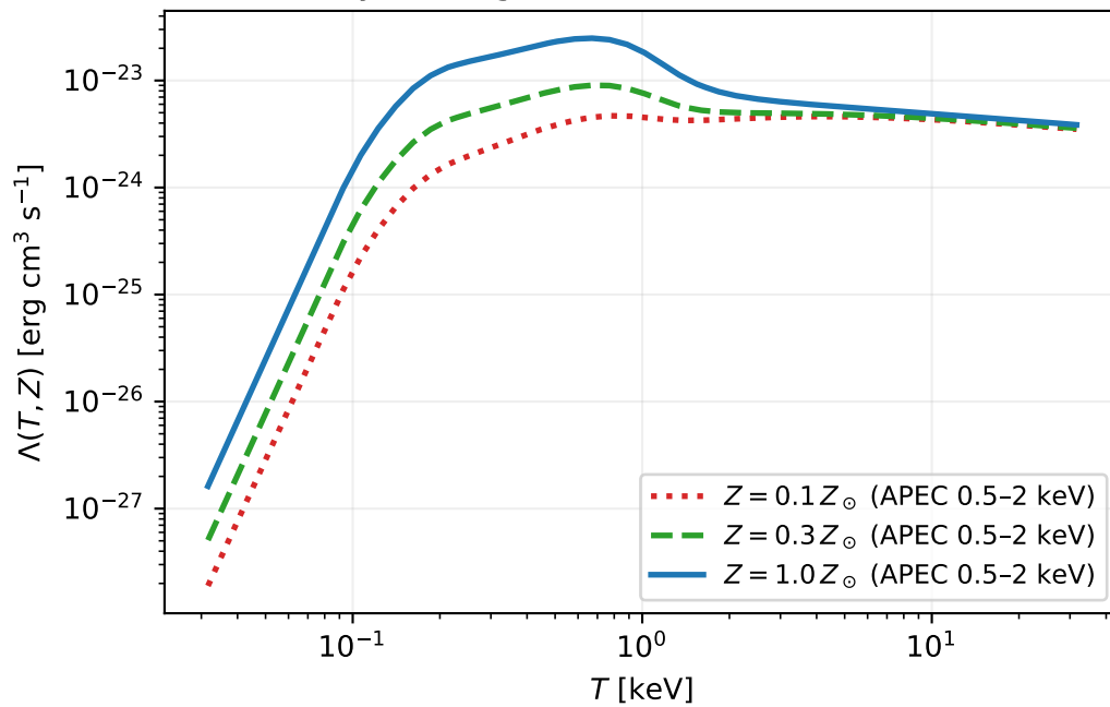
X-ray cooling function (APEC table, soxs)
