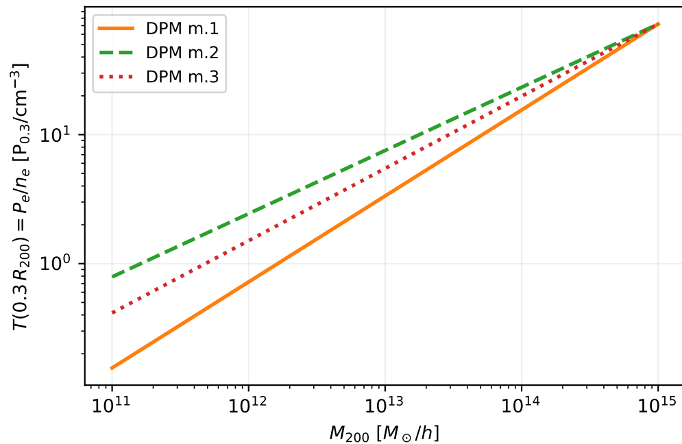
Temperature amplitude at r = 0.3 R_{200} , z = 0.1
