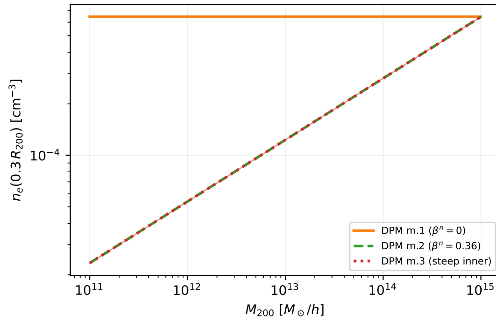
Density amplitude at r = 0.3 R_{200} , z = 0.1
