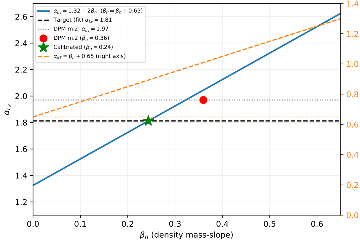
Analytical: L_X \propto M^{1+1.5\beta_n+0.5\beta_p} ( \beta_p = \beta_n + 0.65 )
