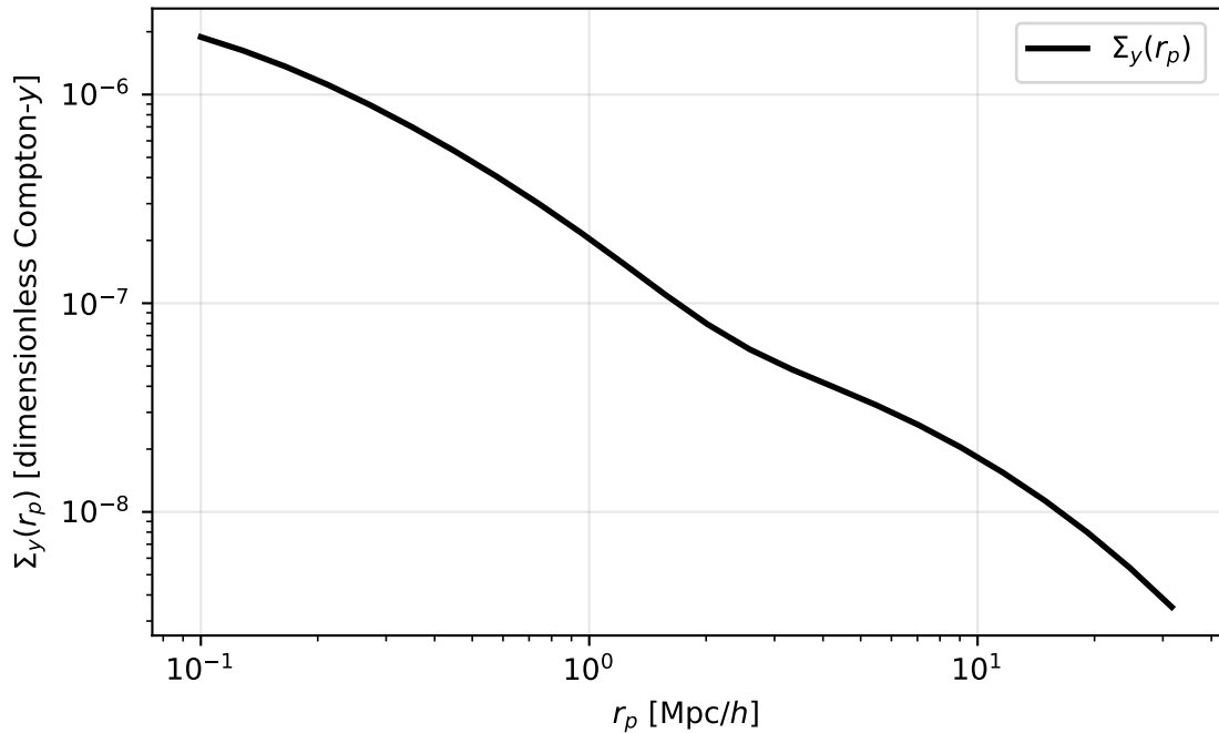
Projected galaxy \times tSZ ( z = 0.3 , A10 pressure)
