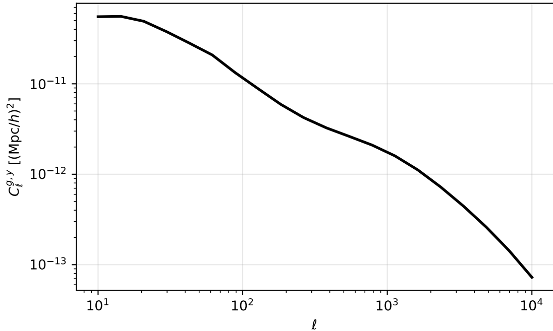
Angular C_\ell^{g,y} (Limber, z \sim 0.3 CMASS-like)
