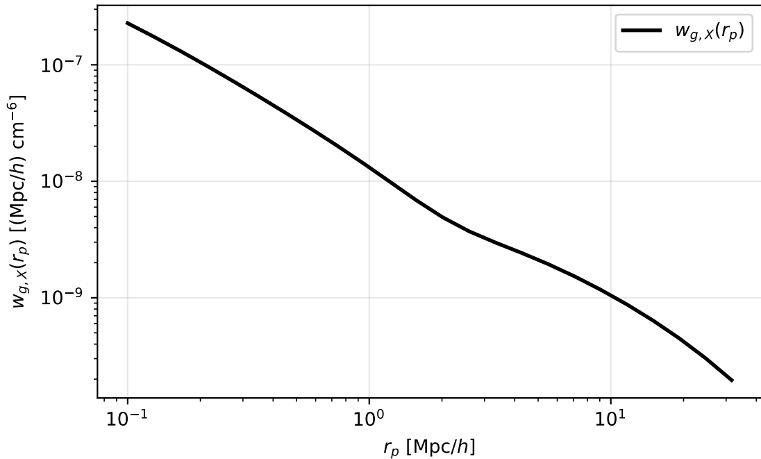
Projected galaxy \times X-ray ( z = 0.3 , DPM Model 2)
