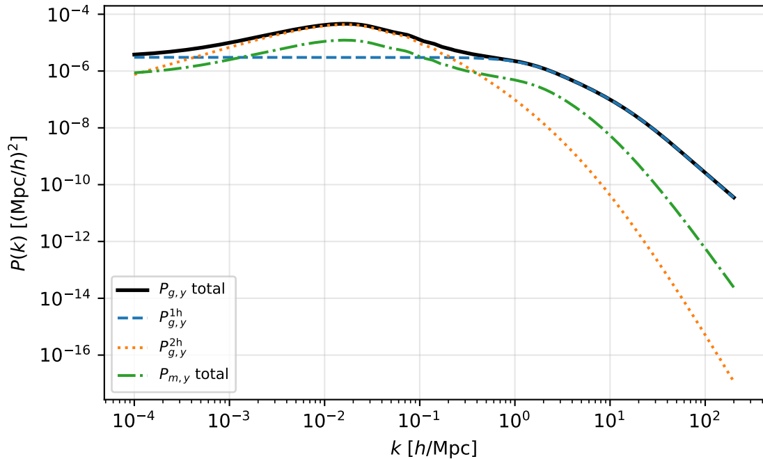
P_{g,y}(k) : CMASS HOD \times A10 pressure, z = 0.55
