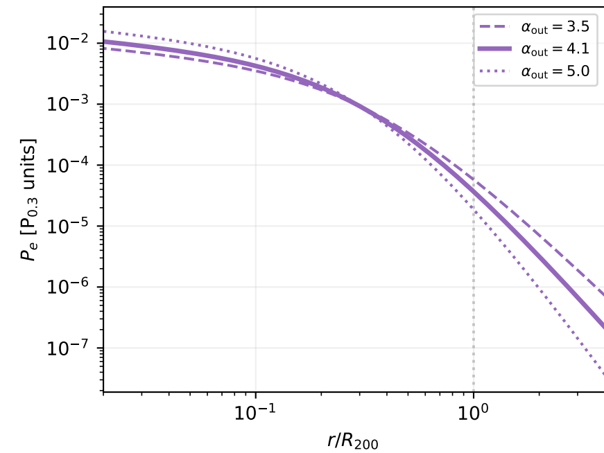
Pressure: vary \alpha_{\text{out}} (outer slope)
