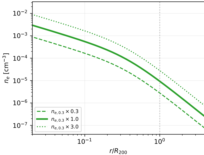
Density: vary n_{e,0.3} (model 2)
