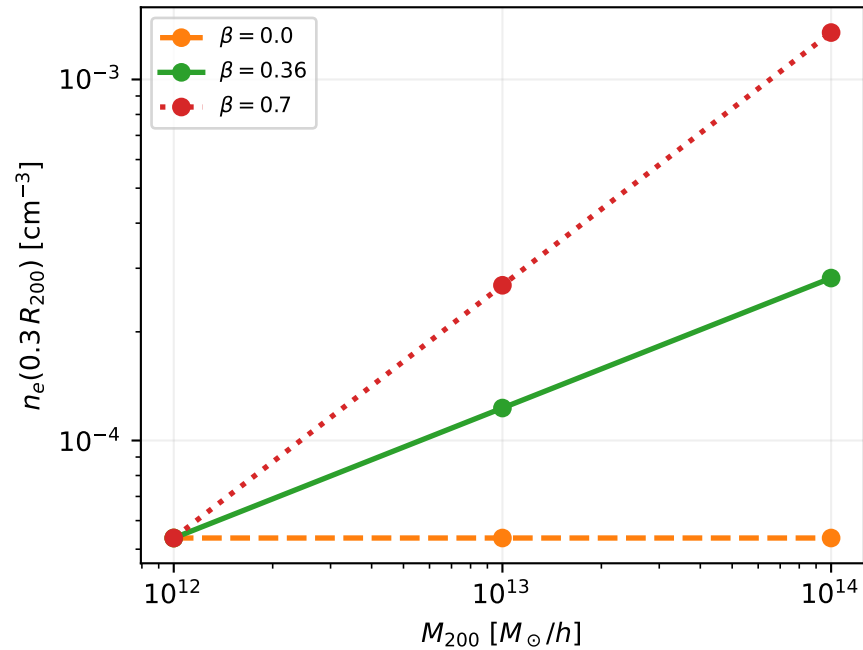
Density: vary \beta (mass scaling)
