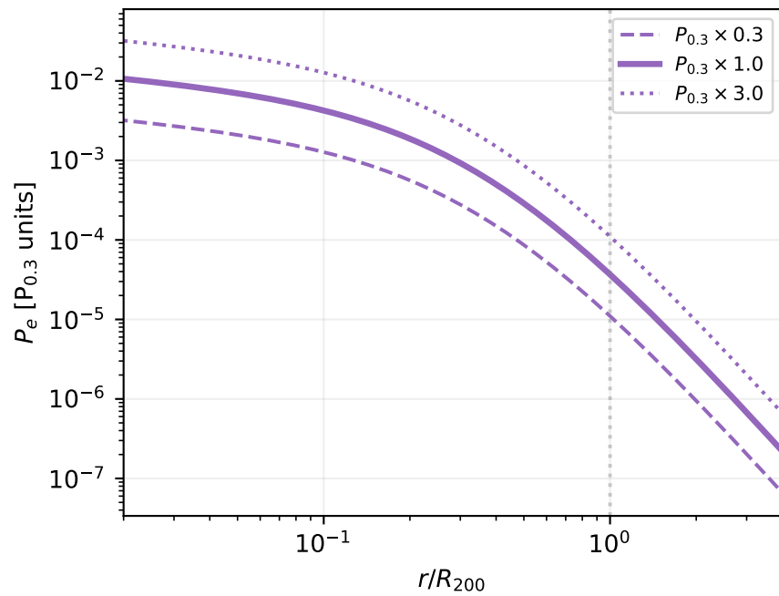
Pressure: vary P_{0.3} (model 2)
