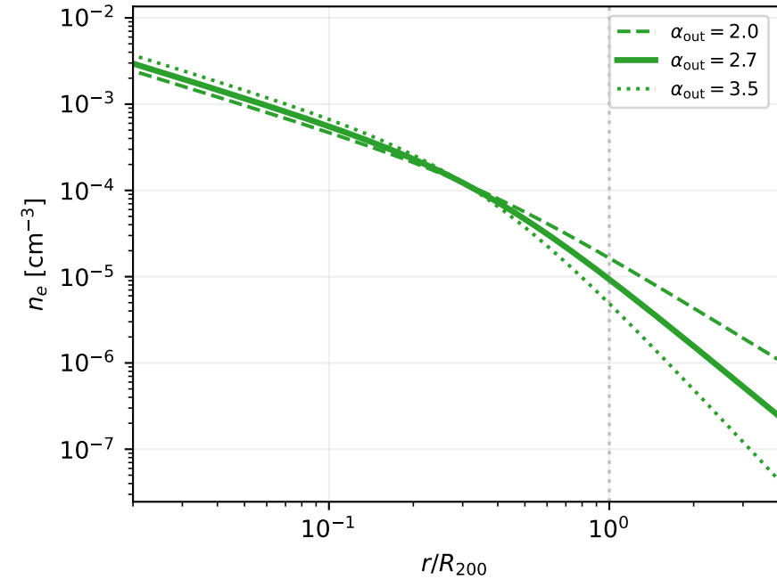
Density: vary \alpha_{\text{out}} (outer slope)
