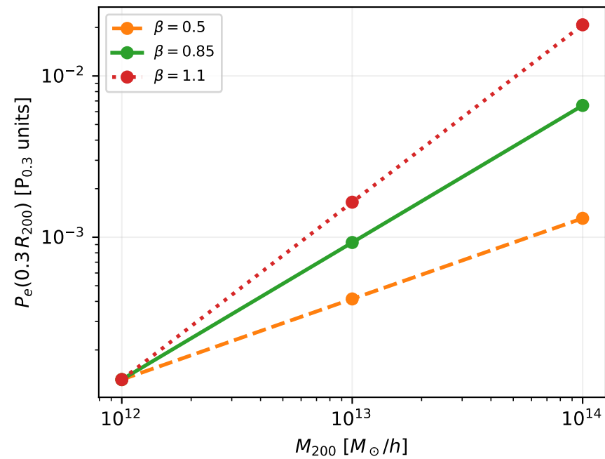
Pressure: vary \beta (mass scaling)
