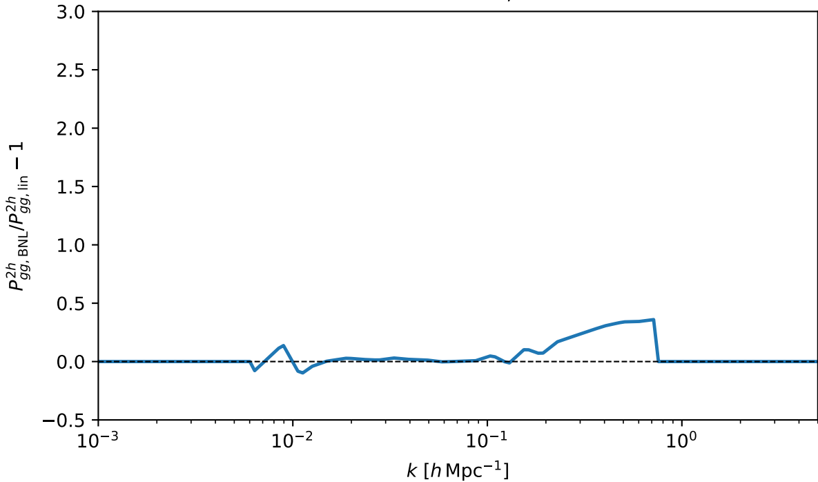
2-halo BNL boost — z = 0.3 , More+2015 HOD
