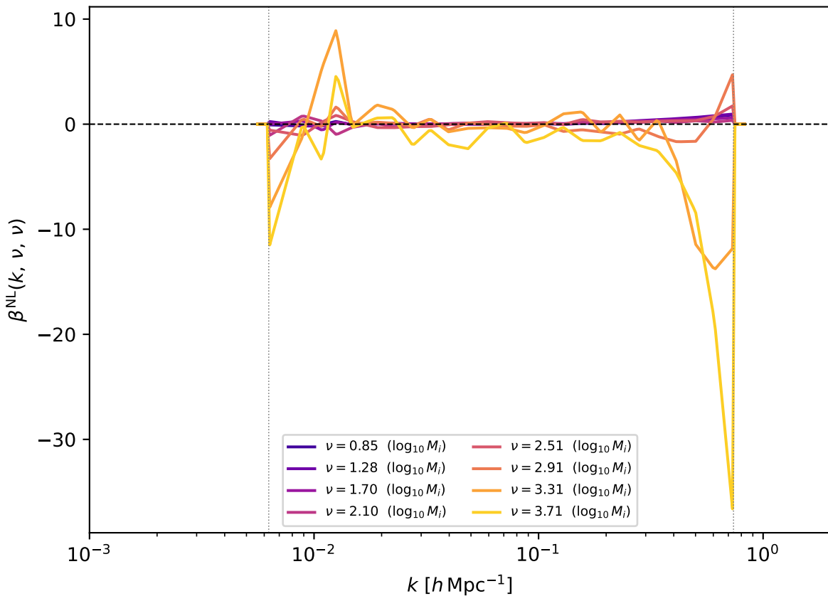
Beyond-linear bias \beta^{\text{NL}} diagonal — Mead \& Verde (2021)
