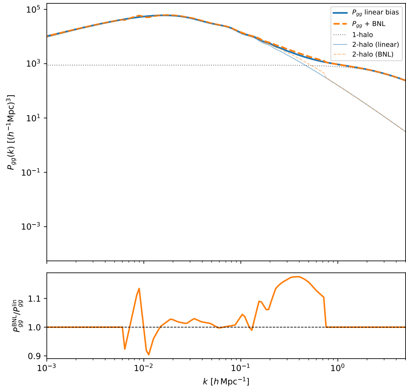
Galaxy power spectrum — z = 0.3 , More+2015 HOD
