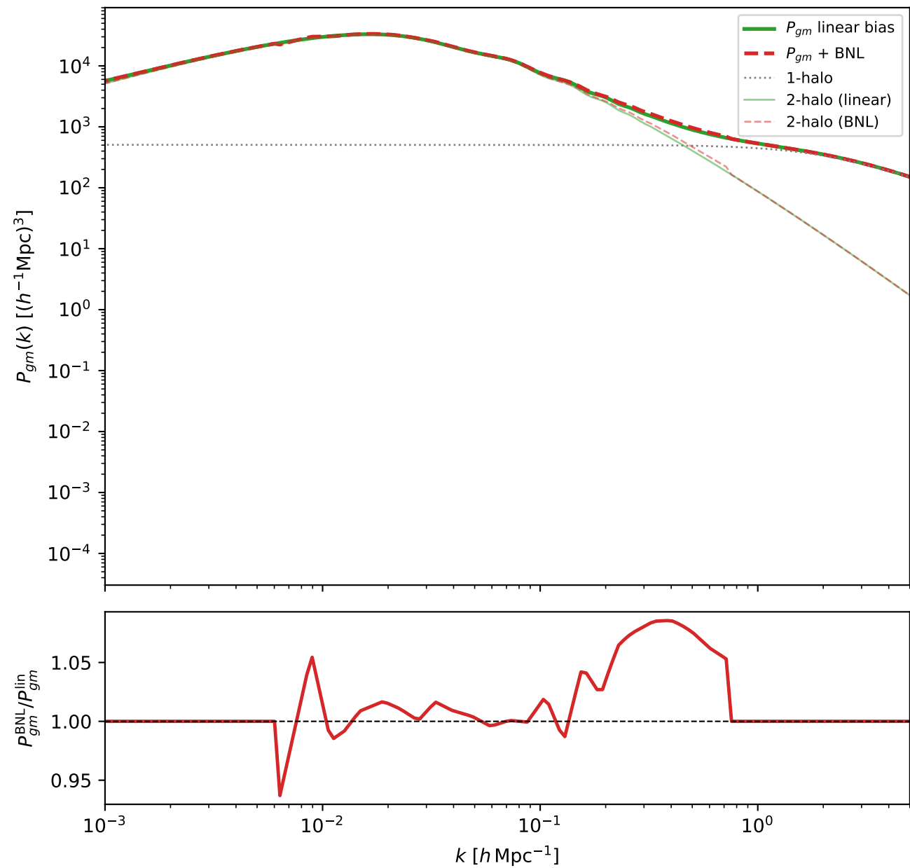
Galaxy-matter cross power — z = 0.3 , More+2015 HOD
