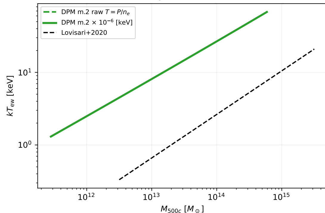
Emission-weighted T : unit correction
