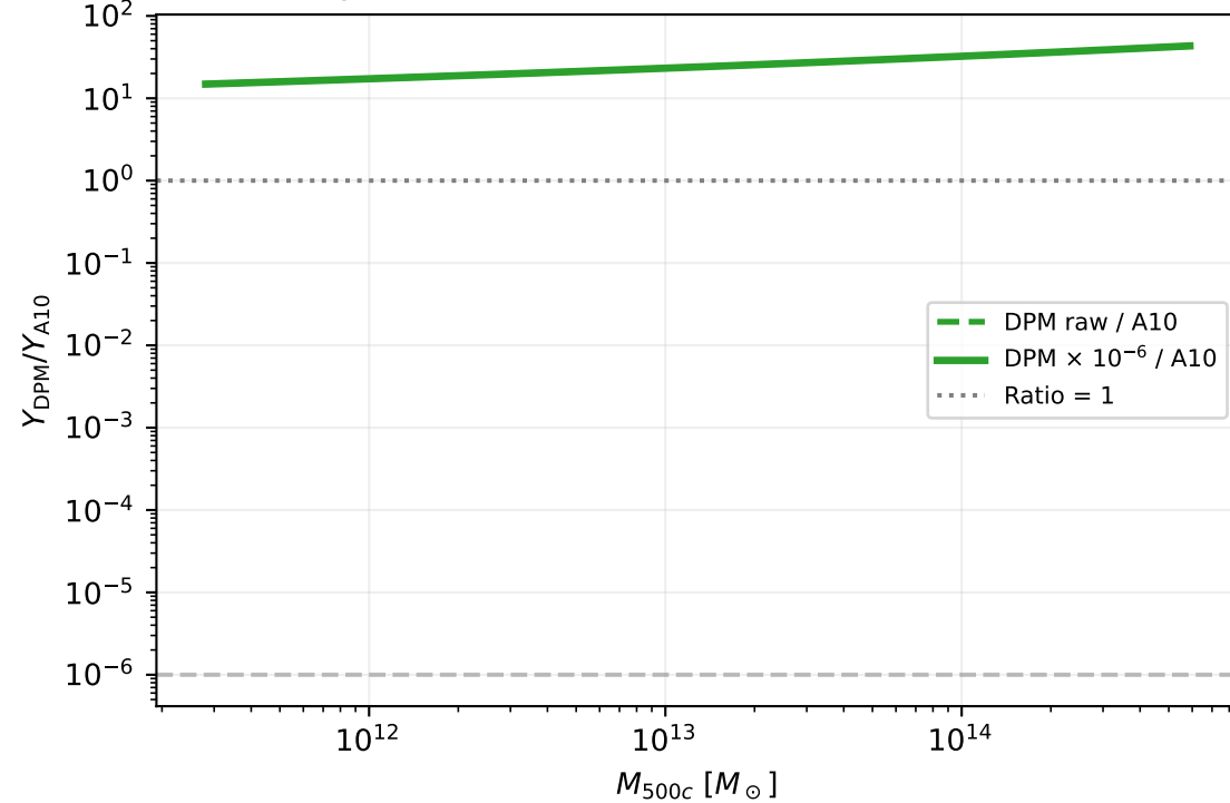
Y_{\text{SZ}} ratio: DPM / A10 (measures unit offset)
