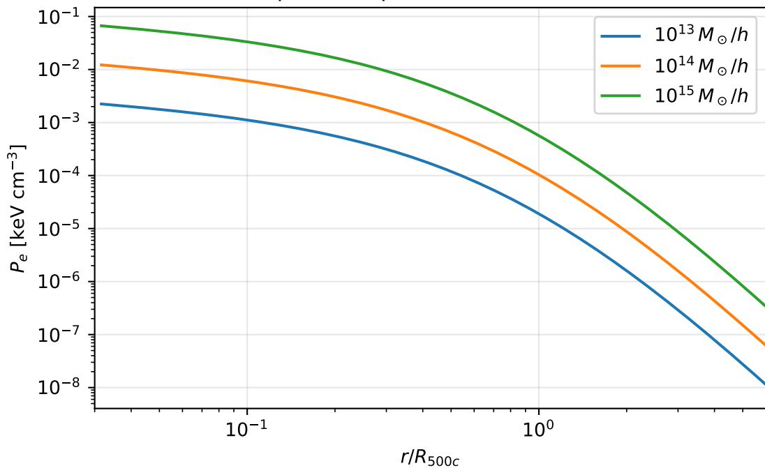
Arnaud+2010 pressure profile (arXiv:0910.1234 Table 1)
