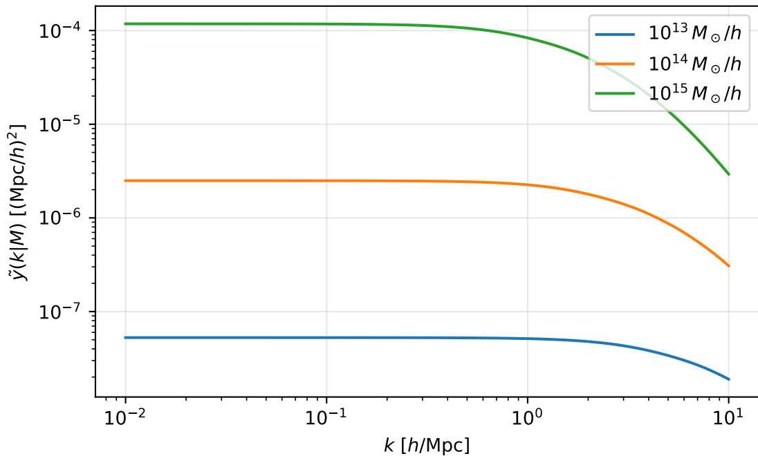
A10 pressure profile FT \tilde{y}(k|M, z = 0.3)
