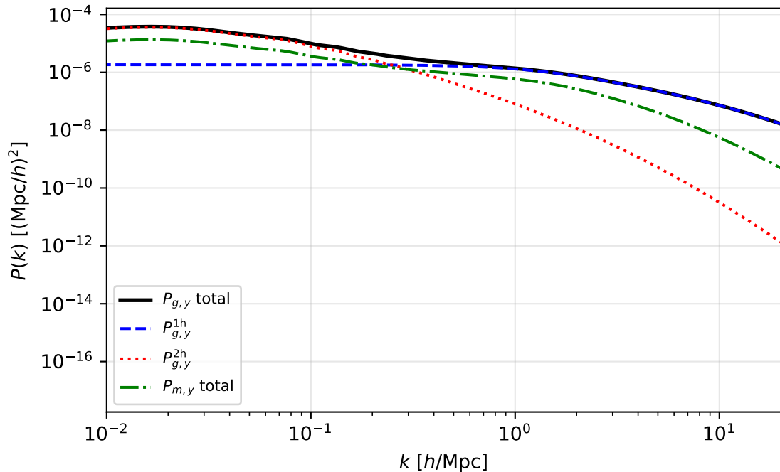
Galaxy \times tSZ power spectrum ( z = 0.3 , A10 pressure)
