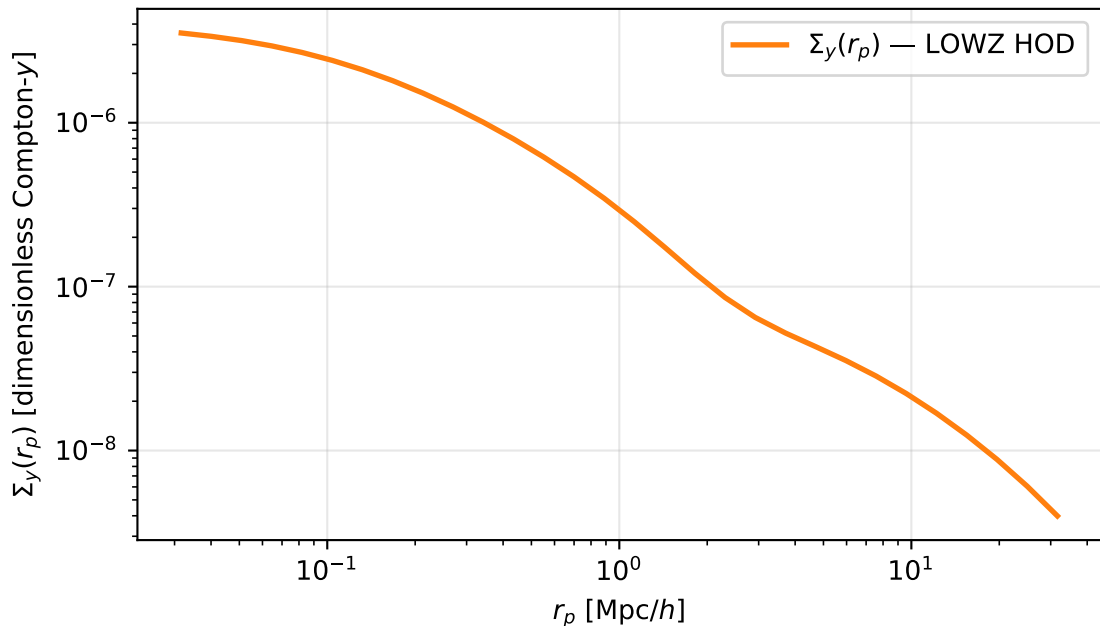
Amodeo+2021 (arXiv:2009.05558) — model tSZ stack, LOWZ z_{\text{eff}} = 0.27 , A10 pressure, More+2015-like HOD
