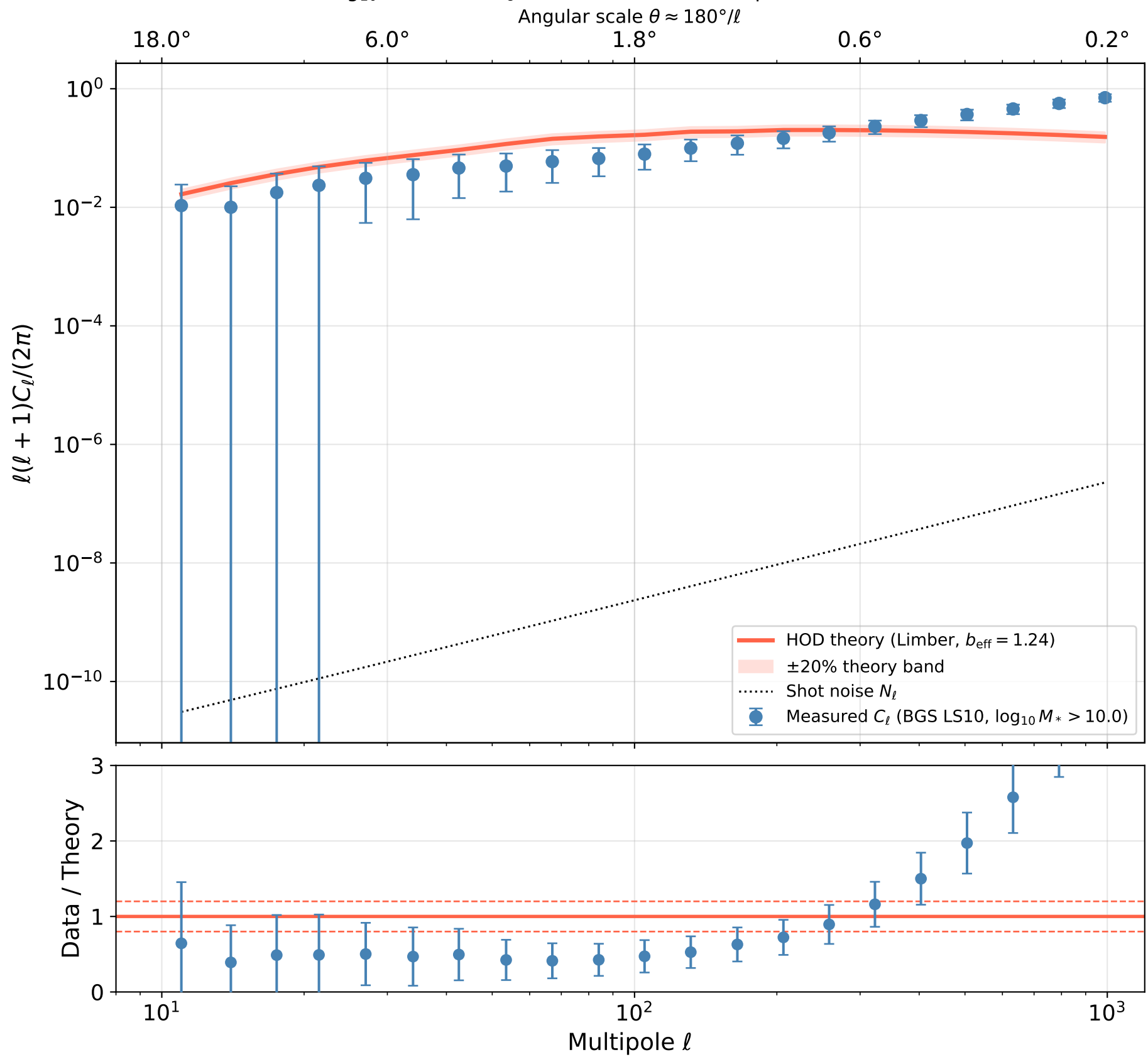
Angular Power Spectrum C_\ell of BGS Galaxies \log_{10} M_* > 10.0 M_\odot , 0.05 < z < 0.18 (Comparat et al. 2025)
