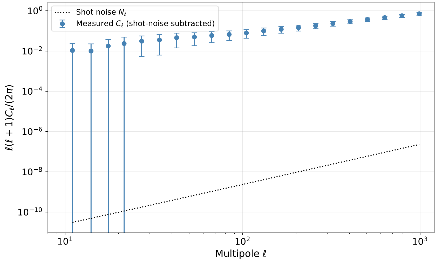
Angular Power Spectrum — BGS LS10 ( \log_{10} M_* > 10.0 , 0.05 < z < 0.18 )
