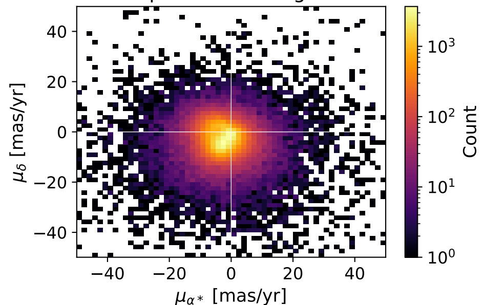
Proper motion diagram
