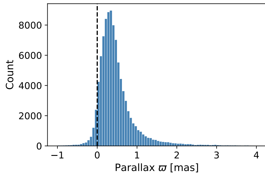
Parallax distribution
