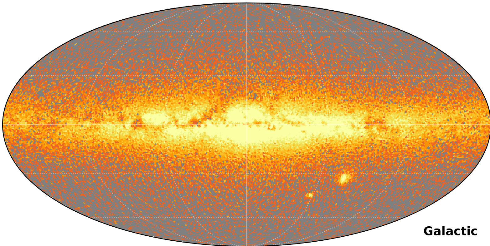
Gaia DR2 Star Density (G=16-17) in Galactic Coordinates Nside=64
