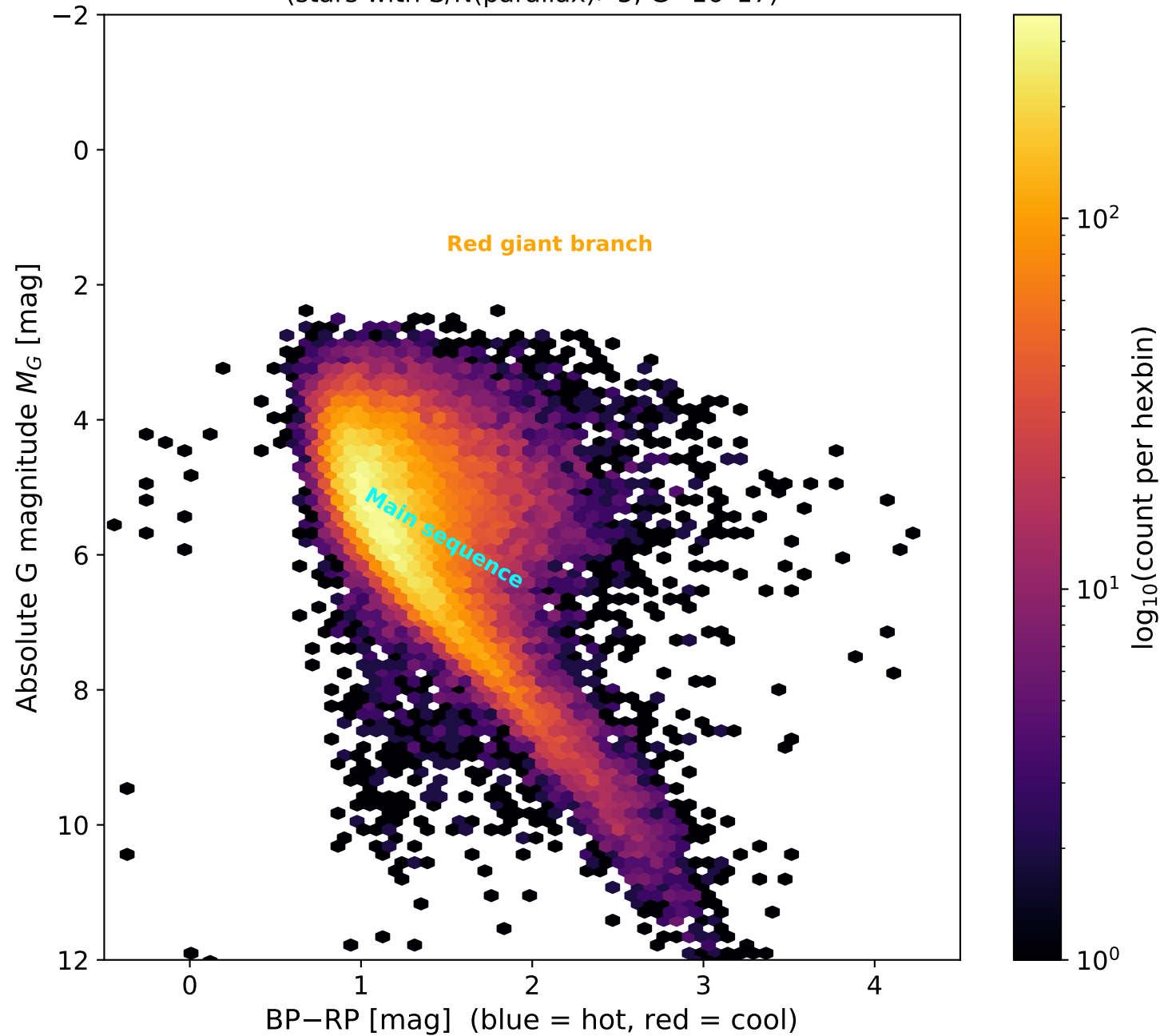
Hertzsprung-Russell diagram from Gaia DR2 (stars with S/N(\text{parallax}) > 5 , G = 16\text{--}17 )
