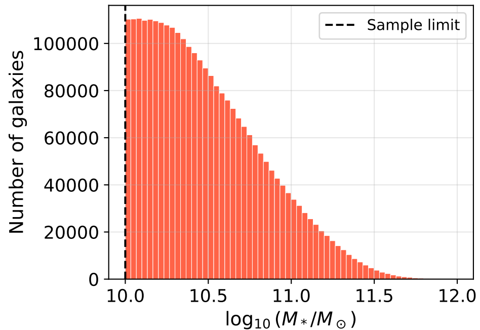
Stellar mass distribution
