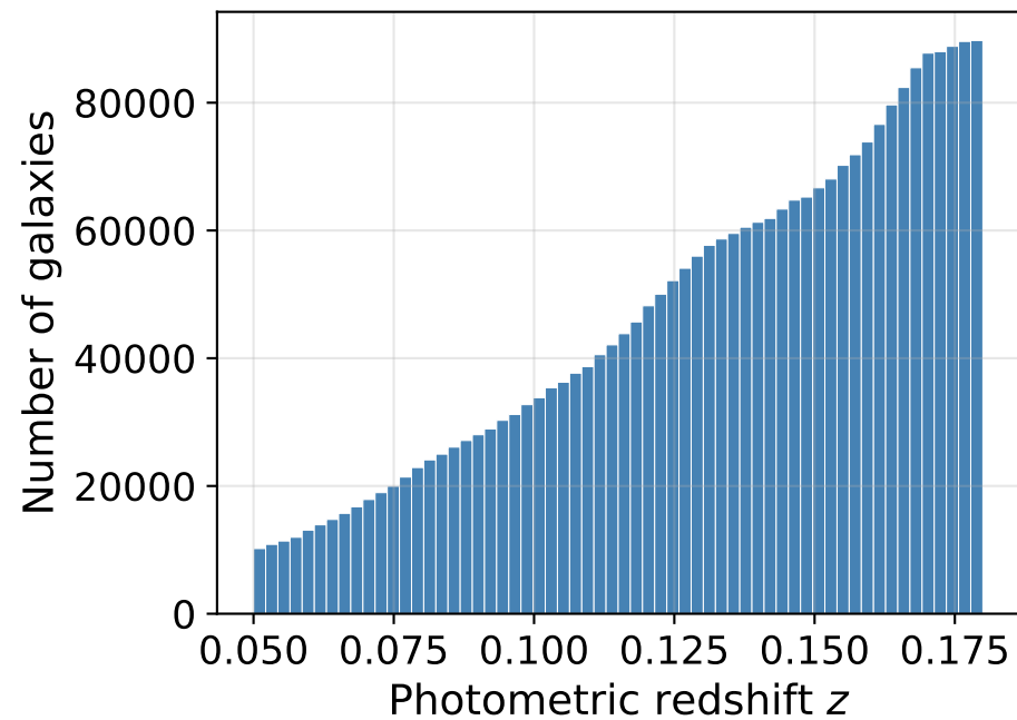
Redshift distribution
