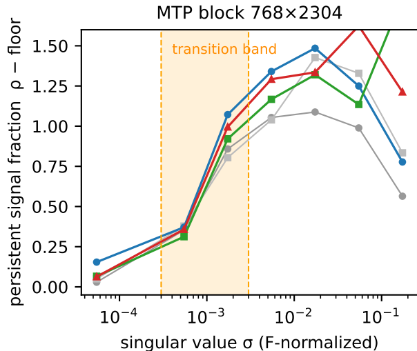
Fig.1 Direction persistence collapses at \sigma^* — and \sigma^* is stationary (MoE, micro-steps 300→1900)
