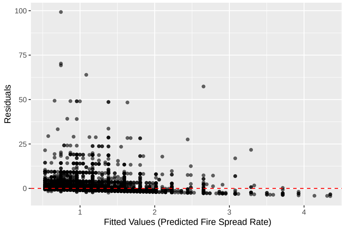
Figure 8: (#fig:residual_plot)Residual Plot
