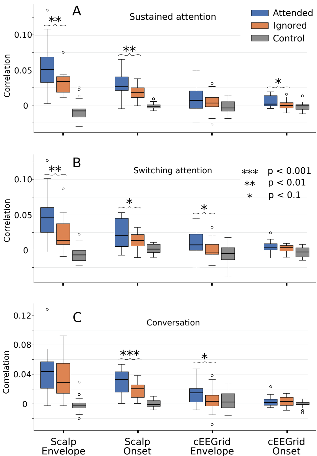
Figure 6: Correlation Analysis: Pearson's correlation between reconstructed and real speech (backward model, 35 s) for SustAC (A), SwitAC (B), and ConvAC (C). The x -ticks indicate electrode type (scalp, cEEGrid) and speech features (acoustic envelope, acoustic onset). Boxplots show attended (blue), ignored (orange), and control (grey) speech, with the median as the black line. Significance stars mark differences of means between attended and ignored speech. No statistical tests were performed between conditions and control speech.
