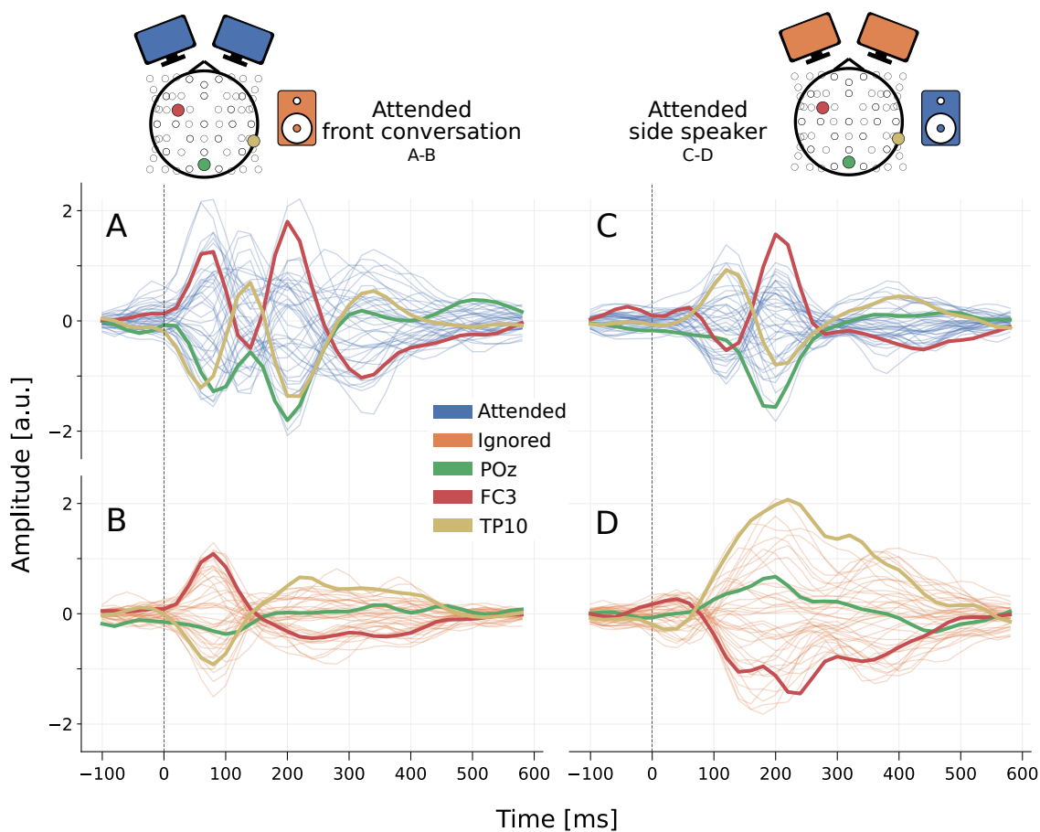
Figure 9: Attention to conversation vs. side talker: conversation attention analysis for trials directed to the front conversation (A-B) and to the side speaker (C-D). Attended speech is shown in blue (A, C) and ignored speech in orange (B, D). Three sensors of interest are highlighted: POZ, FC3 and TP10. All TRFs use the acoustic envelope using scalp EEG.
