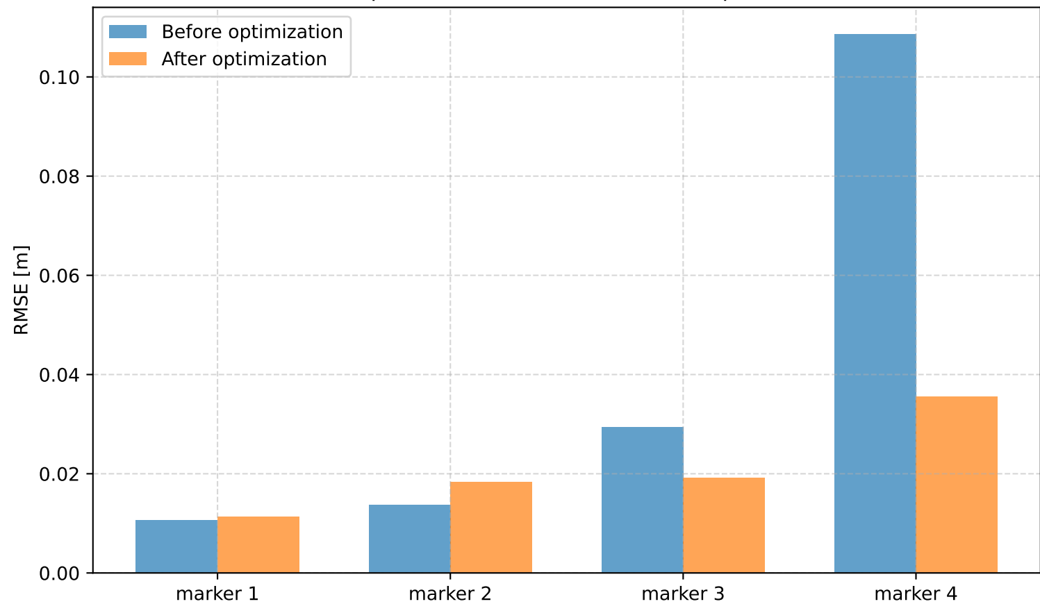
Marker position errors before vs after optimization
