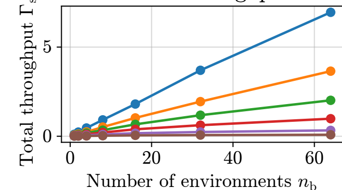
Spatial PCS Total Throughput
