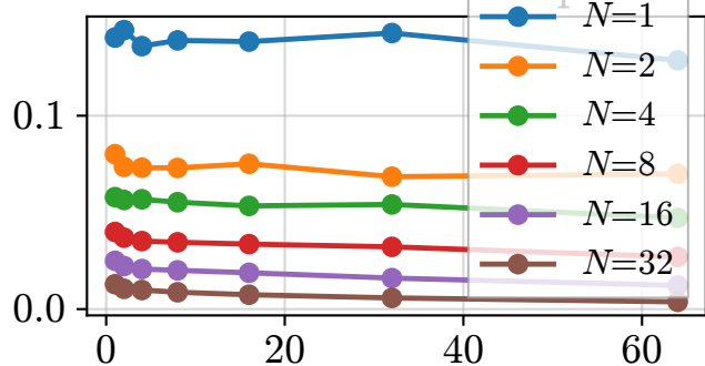
Planar PCS Total Throughput
