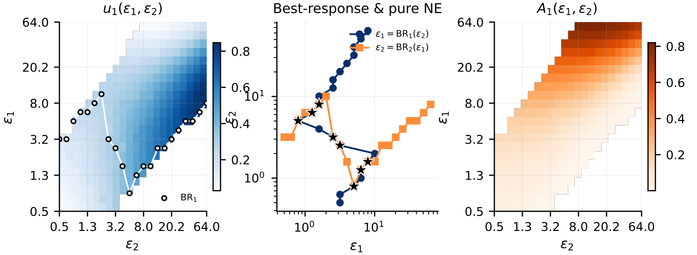
Fig. 1: C1: 2-player payoff u_1(\epsilon_1, \epsilon_2) (left), best-response curves and pure NEs (centre), and realised MIA advantage A_1 (right) on the log-spaced action grid. Infeasible profiles (where any player’s sampling rate falls below the participation threshold) are masked white. The black stars in the centre panel mark pure Nash equilibria, found at the intersection of the two best-response curves. Both equilibria sit off the diagonal of the action grid, confirming that the symmetric pure NE does not exist in this canonical setting.
