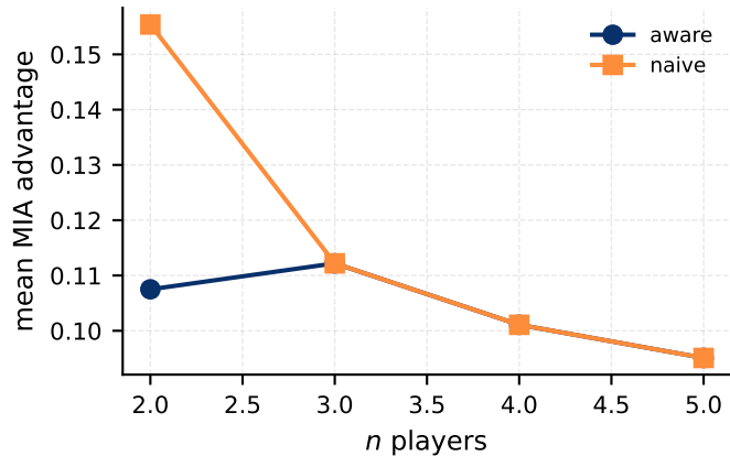
Realised excess vulnerability
