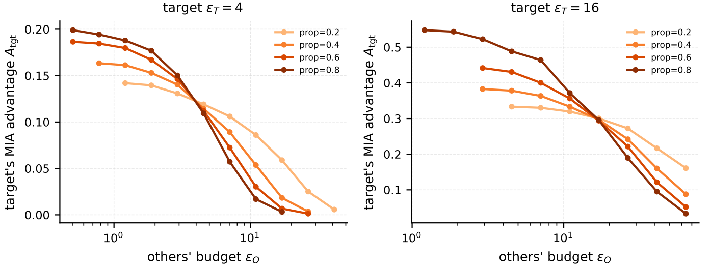
Fig. 4: C5 . Target’s realised MIA advantage as a function of the other group’s budget \varepsilon_O and proportion, at two fixed target budgets \varepsilon_T \in \{4, 16\} . The curves cross at \varepsilon_O = \varepsilon_T . Below crossover, larger proportions raise A_t ; above crossover, larger proportions lower it.
